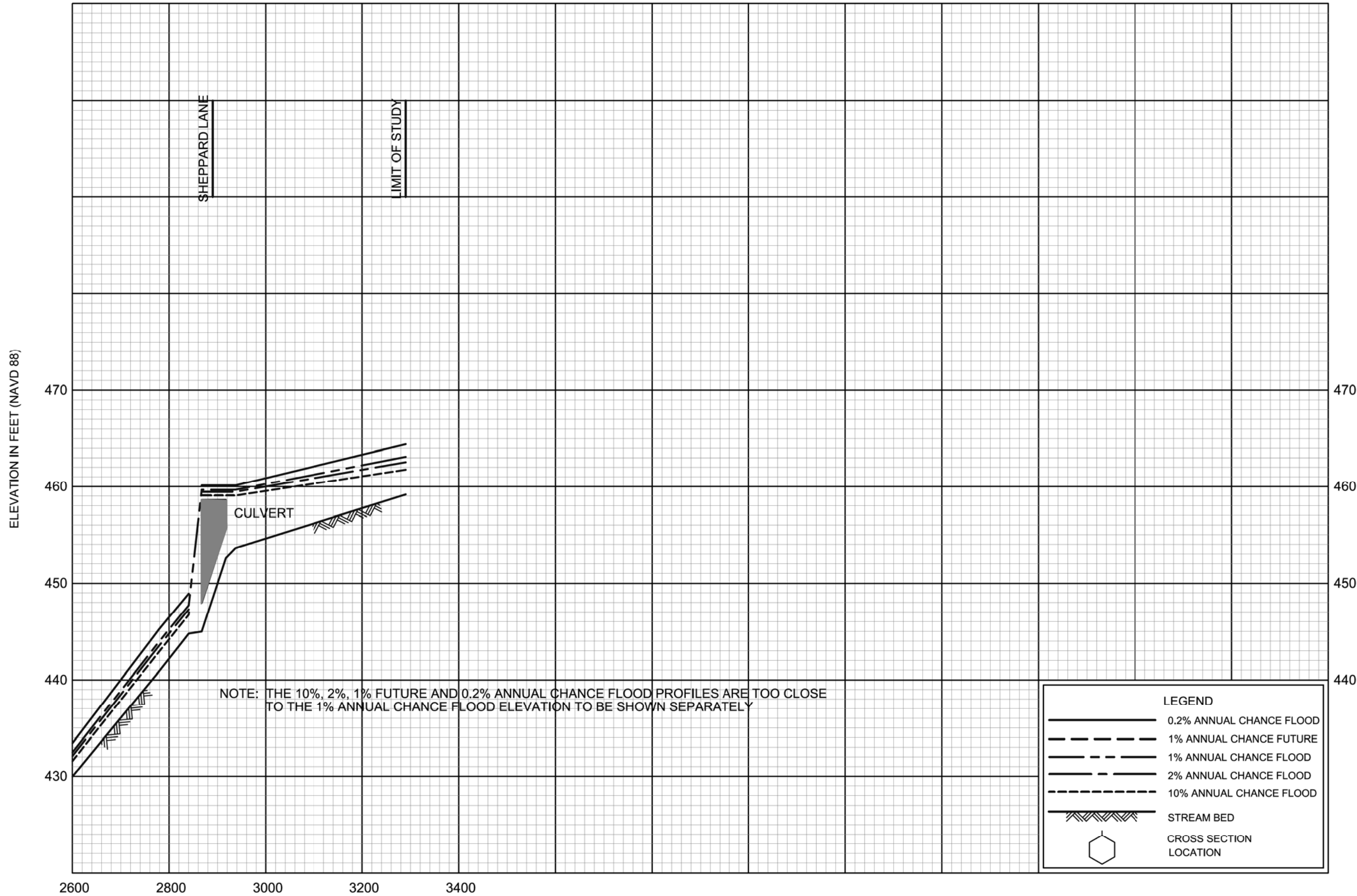
STREAM DISTANCE IN FEET ABOVE CONFLUENCE WITH STREAM CB-1
