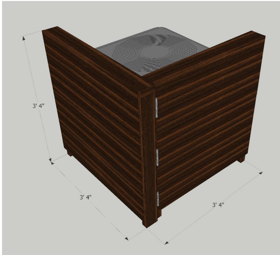
AC Screen Dimensions
