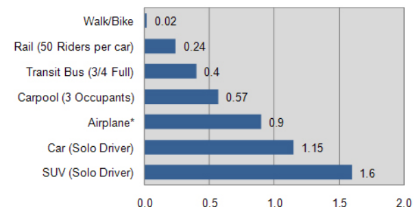
Figure 7.2 Pounds of CO 2 per Passenger Mile
