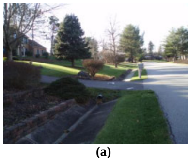
Figure 3.13. (a) Concrete channels could be retrofit to treat stormwater at NSA_27.
