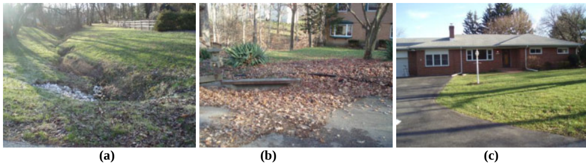
Figure 3.8. Neighborhood NSA_25 with high pollution severity and high restoration potential. (a) Degraded stream reach is potential for stream restoration or buffer enhancement projects; (b) Street sweeping opportunity; and (c) Downspout connected to driveway could be disconnected to pervious lawn.
