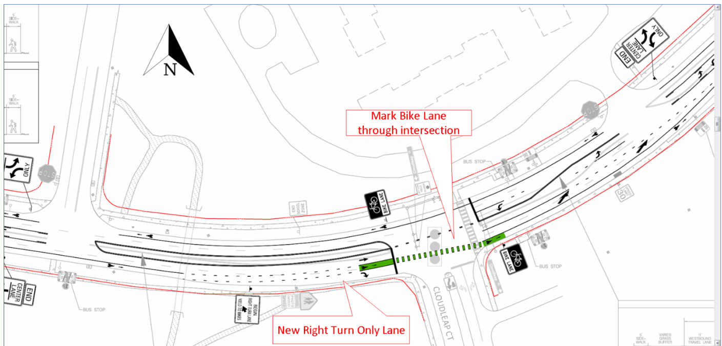
Figure 14: How bike lanes are proposed through the Cloudleap Court
