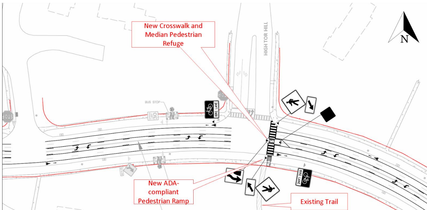
Figure 12: New crossing at High Tor Hill
