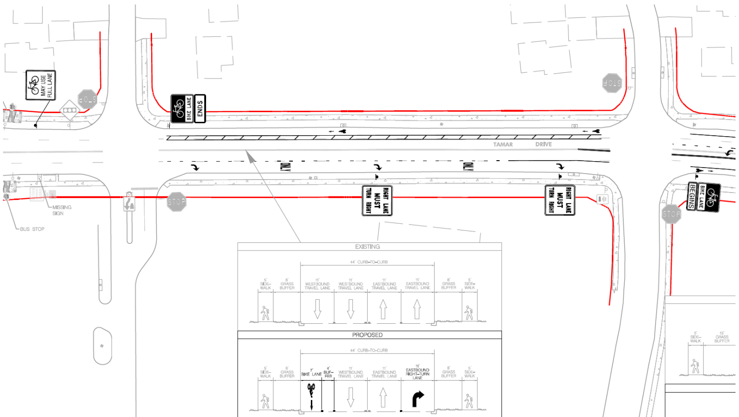
Figure 9: Bike lane termination and beginning at the western project limits
