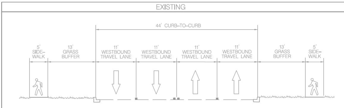
Figure 2: Existing typical section for Tamar Drive
