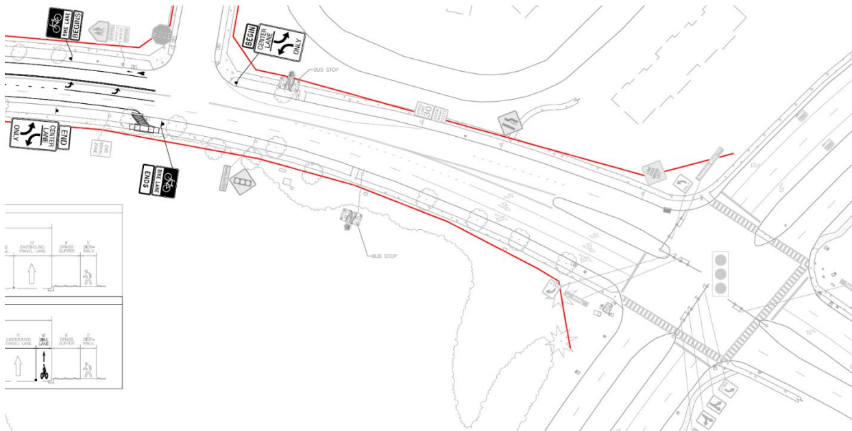
Figure 10: Option 1, eastbound bike lane ends with curb cut and bike ramp to sidewalk
