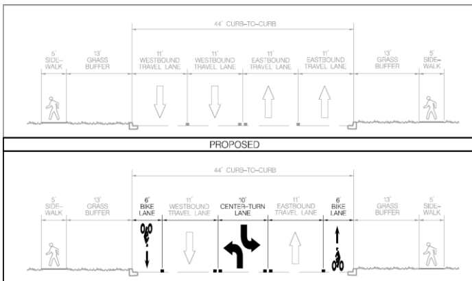
Figure 7: Existing and proposed typical cross-section for Tamar Drive
